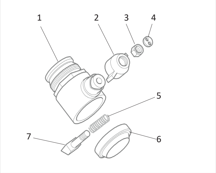
Instantaneous connector assembly - Aluminium 56559 Gunmetal 56559/01
