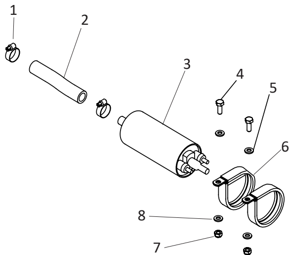
Fuel pump kit - 68247/003
