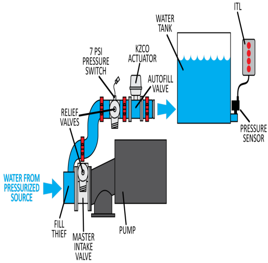
Autofill System with Fill Thief
